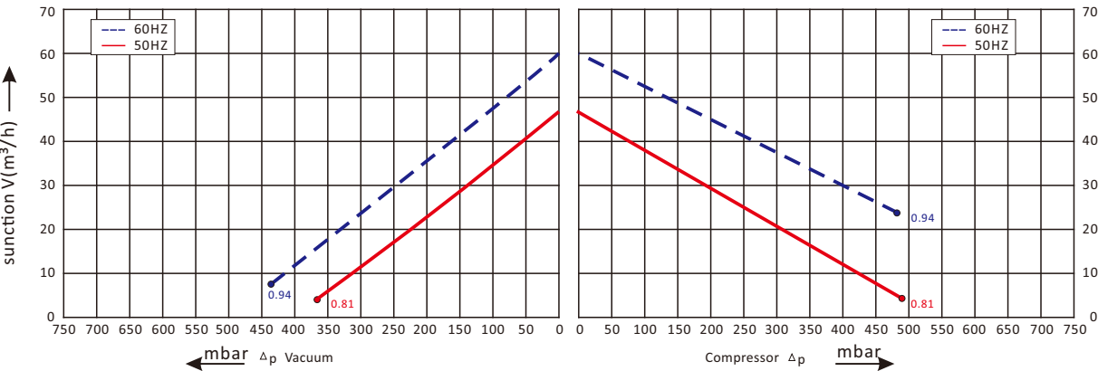
Vacuum selection diagram curve
