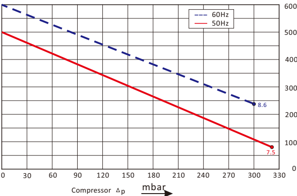
Compressor selection diagram curve
