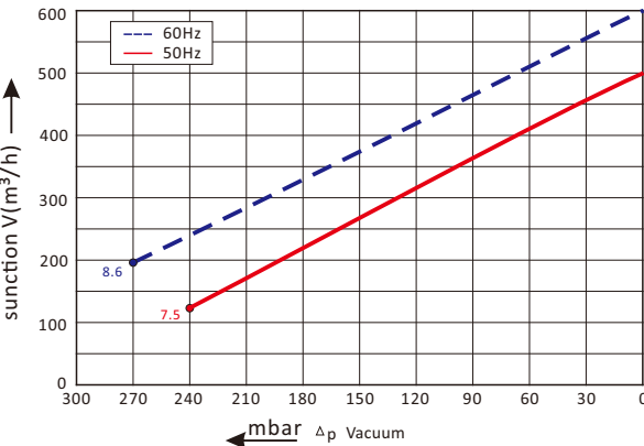
Vacuum selection diagram curve
